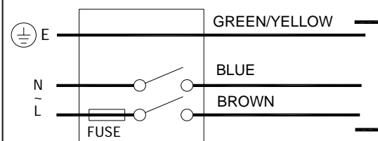
Wiring Diagram for Single Phase Supply (230VAC 50Hz)
